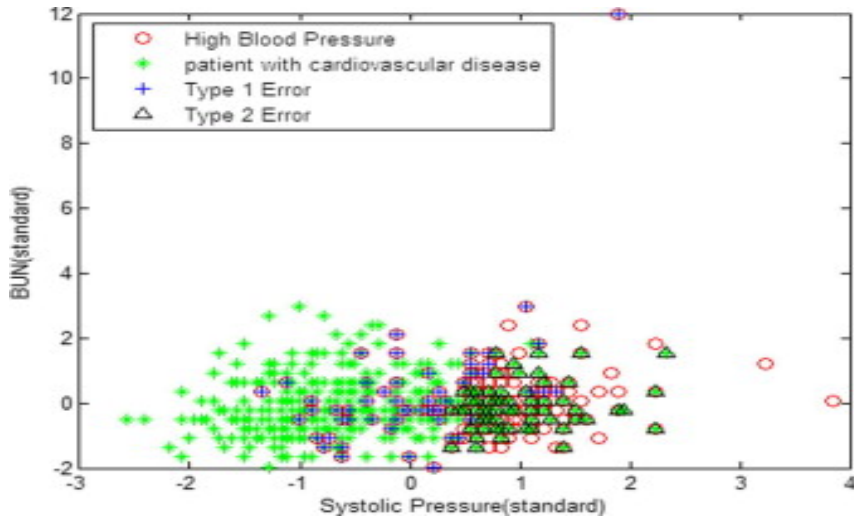
Figure 4. K-NN Classifier for Chronic Disease [39]
